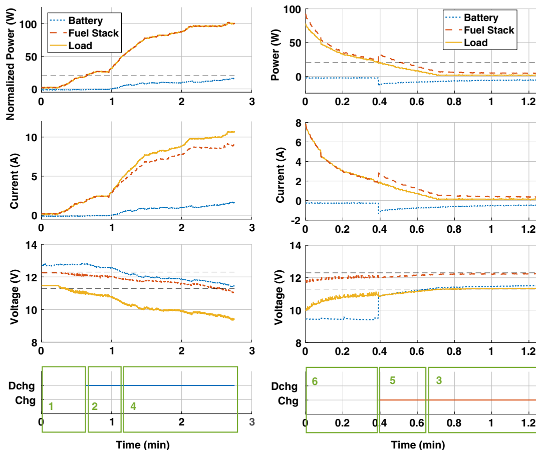
Fig. 12 Demonstration of power sharing circuit's six operating modes.
