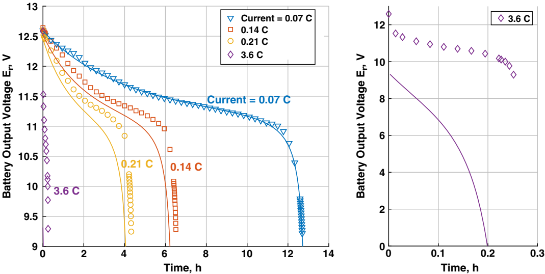
a) Discharge model compared to experimental data b) Close-up view of small time range Fig. 5 Shepherd model compared to test data; model parameters extracted at 0.07 C.
