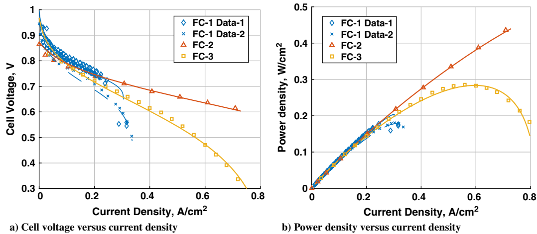
Fig. 2 Steady-state characteristics of three different fuel cells (FC-1 through FC-3 defined in text): data and models.
