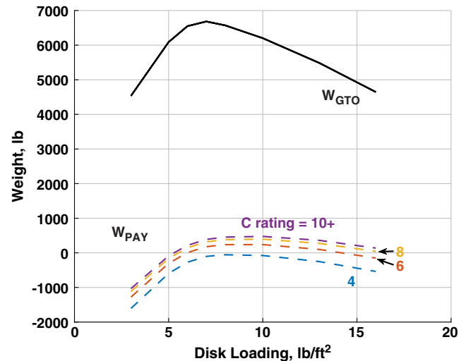
Fig. 25 Aircraft payload and gross take-off weights as a function of disk loading B-FC hybrid powered; baseline technology; tilting prop rotor.
