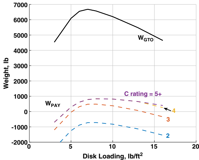
Fig. 32 Aircraft payload and gross take-off weights as a function of disk loading battery only; baseline technology; tilting proprotor; shortest intracity mission.
