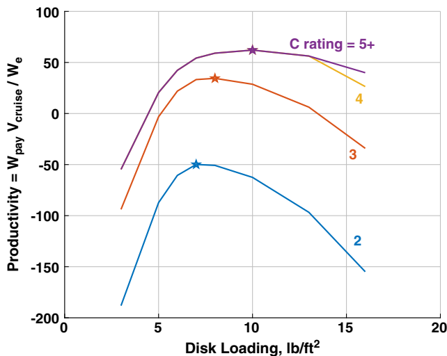
Fig. 33 Aircraft productivity as a function of disk loading fuel cell versus battery; baseline technology; limited battery C rating; tilting proprotor; shortest intracity mission.
