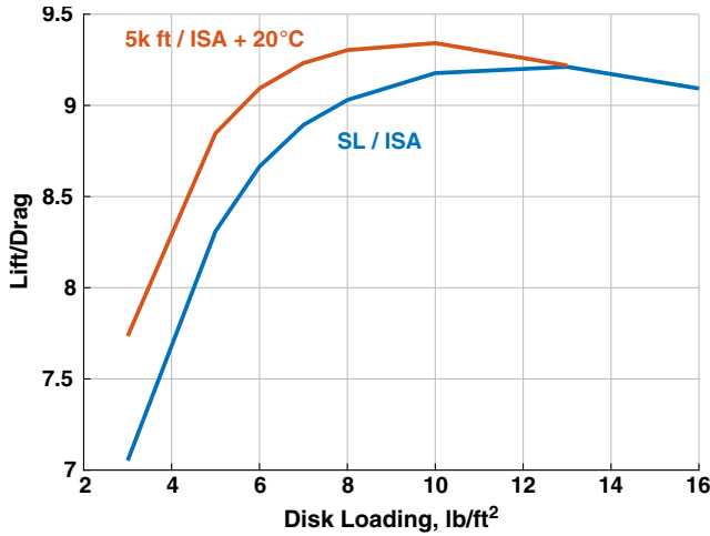
Fig. 18 Maximum lift-to-drag ratio versus disk loading for final aircraft designed for 75 mile range; at cruise tip Mach number of 0.28.
