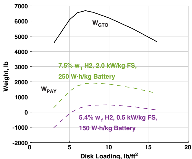
Fig. 23 Aircraft payload and gross take-off weights as a function of disk loading B-FC hybrid powered; baseline technology; tilting prop rotor.
