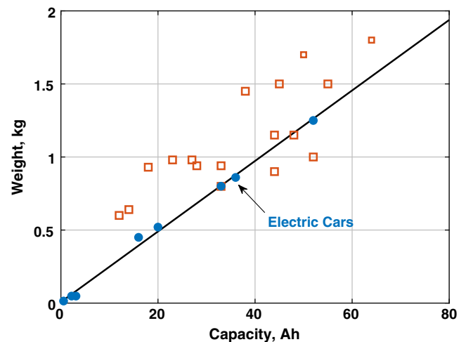
Fig. 15 Lithium–ion cell weights versus capacity in ampere hours.
