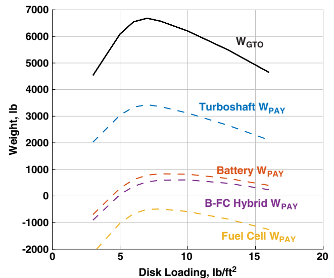
Fig. 30 Aircraft payload and gross take-off weights as a function of disk loading various powerplants; baseline technology; tilting propotor; shortest intracity mission.
