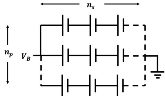
Fig. 14 Schematic of batteries or fuel cells connected in series and parallel.
