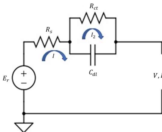
Fig. 3 Basic equivalent circuit network of fuel cell.
