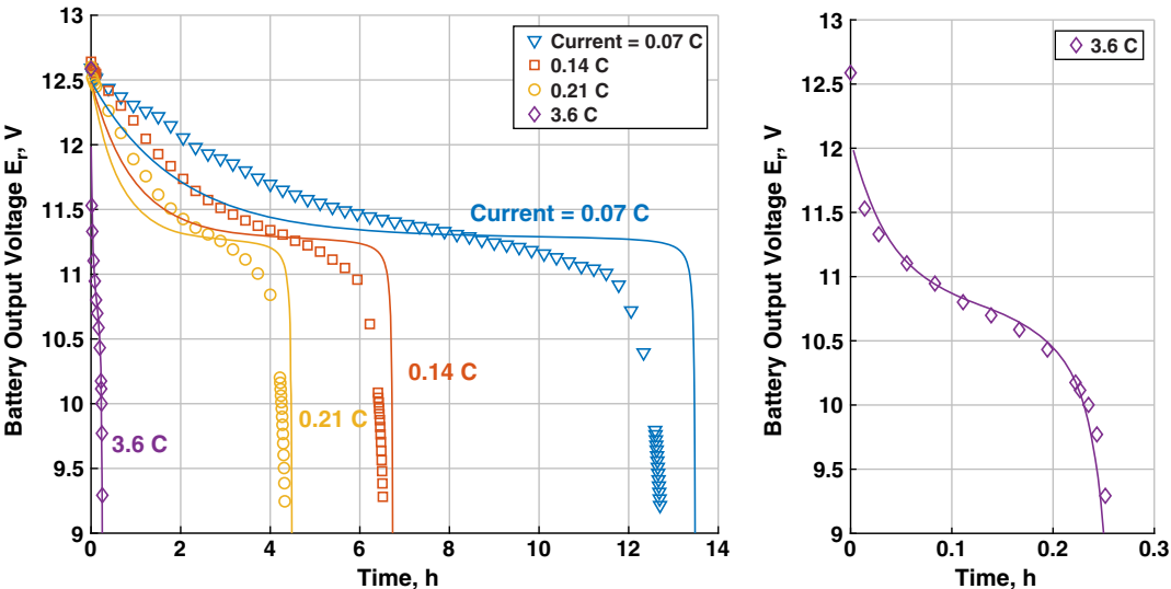
a) Discharge model compared to experimental data b) Close-up view of small time range Fig. 6 Shepherd model compared to test data; model parameters extracted at 3.6 C.
