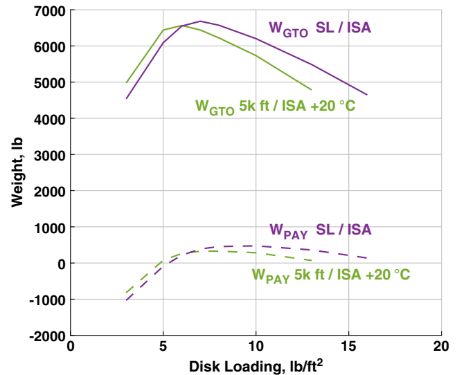
Fig. 24 Aircraft payload and gross take-off weights as a function of disk loading B-FC hybrid powered; high-altitude and -temperature comparison; baseline technology; tilting prop rotor.
