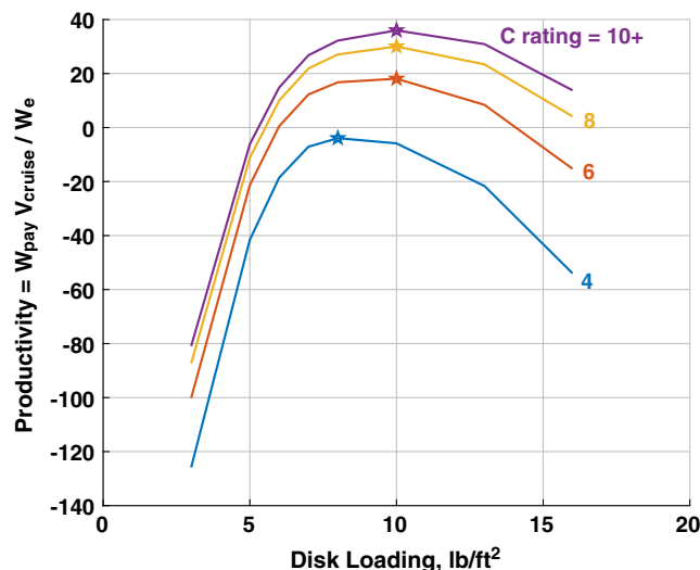
Fig. 26 Aircraft productivity as a function of disk loading B-FC hybrid powered; baseline technology; tilting proprotor.
