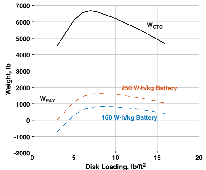
Fig. 31 Aircraft payload and gross take-off weights as a function of disk loading battery-only powerplant; improved technology comparison; tilting propotor; shortest intracity mission.
