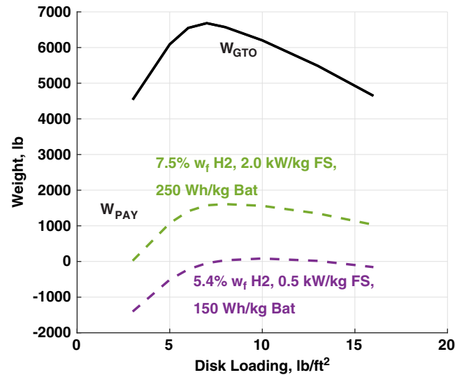
Fig. 28 Aircraft payload and gross take-off weights as a function of disk loading B-FC hybrid power; improved technology comparison; tilting propotor; extended range mission.
