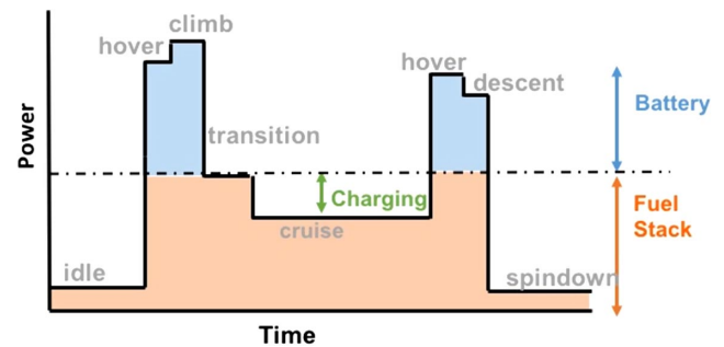
Fig. 10 Power supplied by fuel stack and battery in regulated operation for a notional mission power profile.
