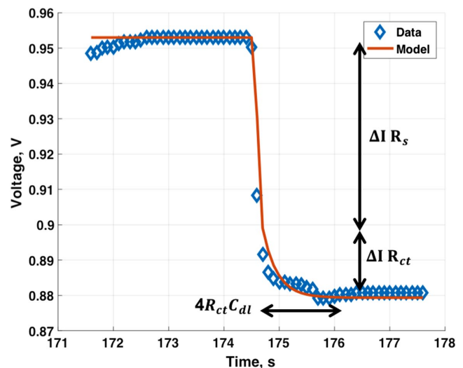
Fig. 4 Voltage response to a step current drawn from a fuel stack.
