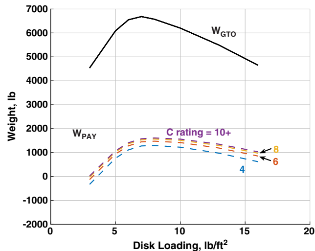
Fig. 29 Aircraft payload and gross take-off weights as a function of disk loading B-FC hybrid; improved technology; tilting propotor; extended range mission.
