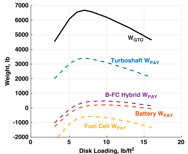
Fig. 20 Aircraft payload and gross take-off weights as a function of disk loading; various power sources; baseline technology; tilting propeller configuration.
