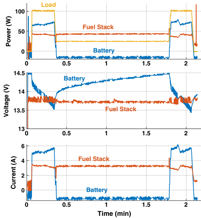
Fig. 13 Power, voltage, and current of battery and fuel stack in regulated parallel configuration; demonstrates ideal power sharing.
