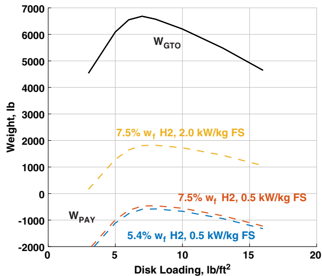
Fig. 22 Aircraft payload and gross take-off weights as a function of disk loading fuel cell powered; improved technology; tilting prop rotor.
