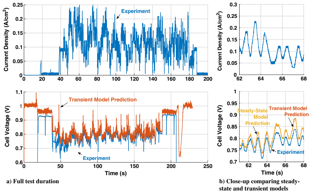
Fig. 7 Model compared to experimental voltage for fuel stack for highly transient load.
