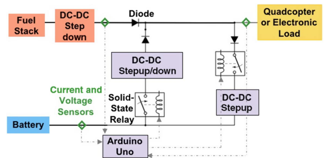
Fig. 11 Circuit schematic for regulated power sharing operation with added Arduino microcontroller, solid-state relay switches, and direct current (DC) converters.
