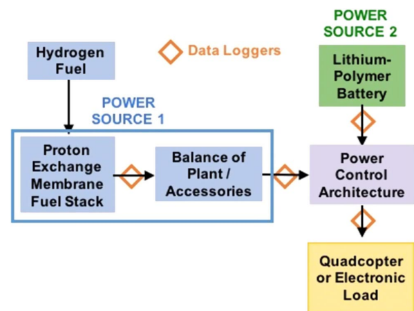
Fig. 1 Flow diagram of a parallel hybrid power system.
