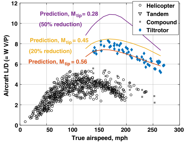
Fig. 17 L/D versus true airspeed of VTOL aircraft; tiltrotor data from XV-15 in cruise mode (zero flaps, pylons down).
