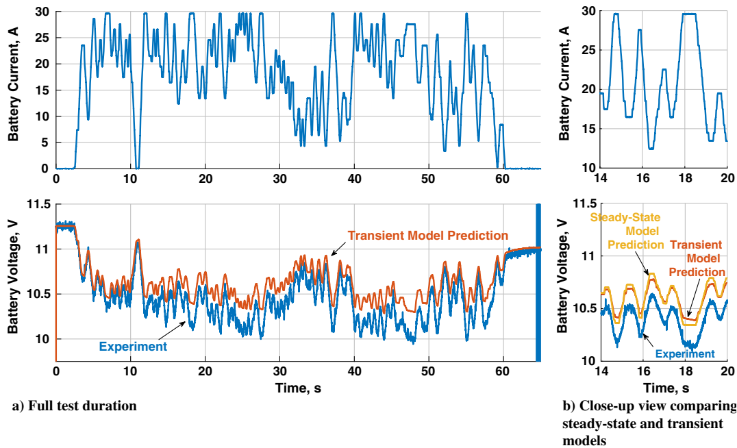
Fig. 8 Model compared to experimental voltage for battery for highly transient load.
