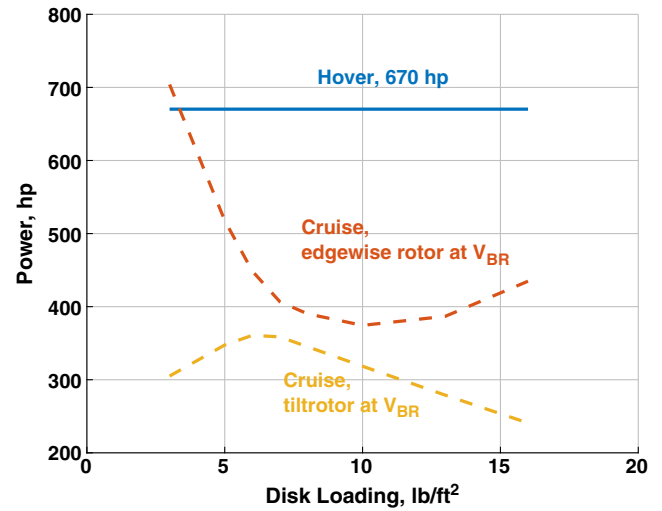
Fig. 19 Cruise power versus disk loading for edgewise and tilting propellers.
