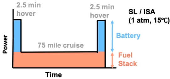
Fig. 16 Baseline power profile used in eVTOL sizing section (Sec. VI) showing B-FC hybrid power sharing scheme.
