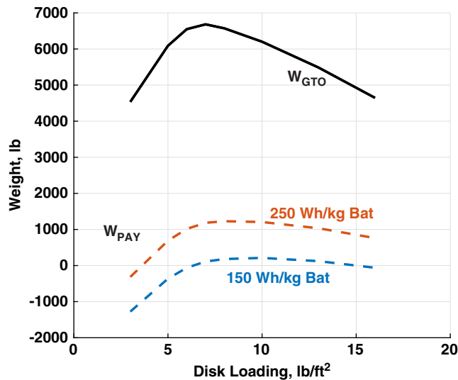
Fig. 21 Aircraft payload and gross take-off weights as a function of disk loading battery powered; improved technology; tilting prop rotor.
