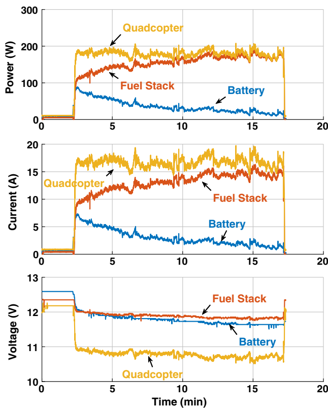
Fig. 9 Experimental power, current, and voltage of battery, fuel stack, and quadcopter during hover.
