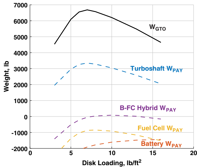
Fig. 27 Aircraft payload and gross take-off weights as a function of disk loading various power sources; baseline technology; tilting propotor; extended range mission.
